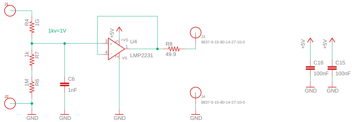
Banana Plug Inputs 1:1000 Divider Low bias current op-amp Tip Jack Outputs Decoupling Cap
