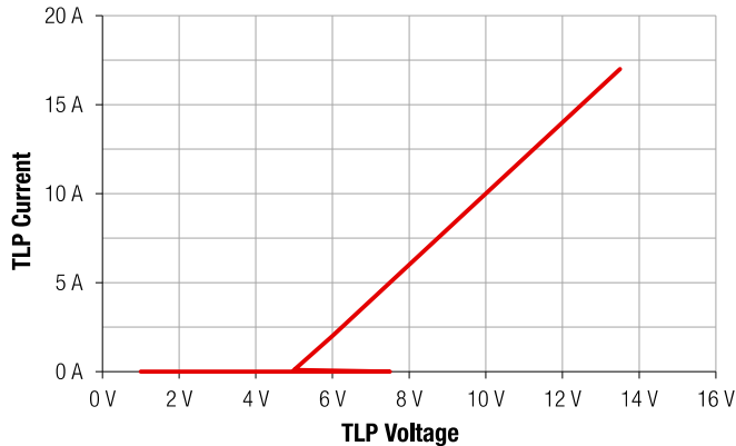
Figure 14: TLP Measurement
